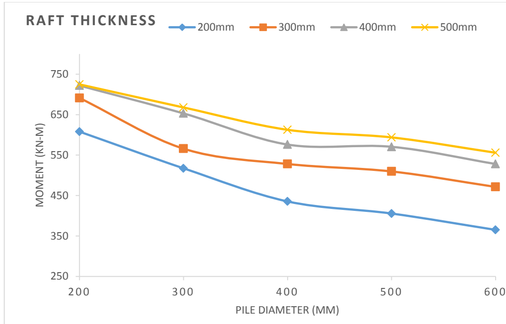
Fig. 8 Variation in maximum moment for piled raft foundation
