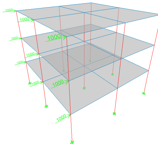
Fig. 2 Typical building frame with fixed base considered in the present investigation
