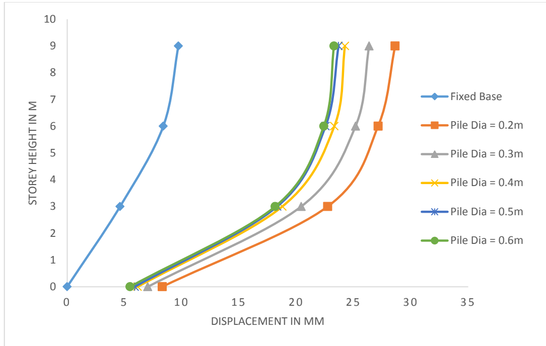
Fig. 6 Effect of pile diameter on displacement
