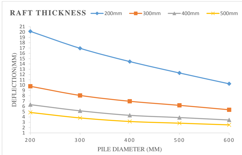
Fig. 7 Variation in maximum displacement for piled raft foundation
