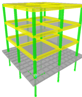
Fig. 5 Mathematical model of frame with piled-raft using ETABS
