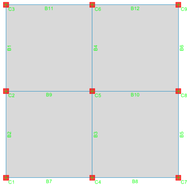
Fig. 3 Particulars of the frame (plan) showing the element numbering for various components of the frame [Top slab]
