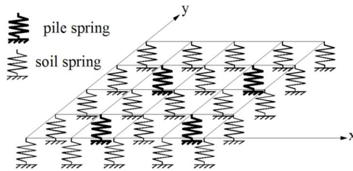
Fig. 1 Structural idealization for piled raft and supporting soil
