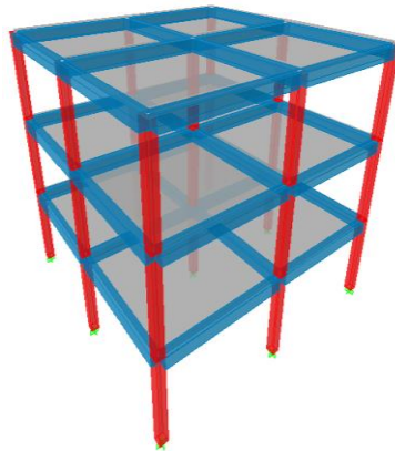
Fig. 4 Mathematical model of frame assuming fixed column bases using ETABS
