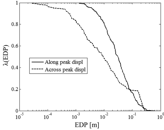
Fig. 4 Sensitivity analyses –set No. 1, assumed random variable V_{10} : mean annual frequencies \lambda(EDP) of exceeding any value of the EDPs
