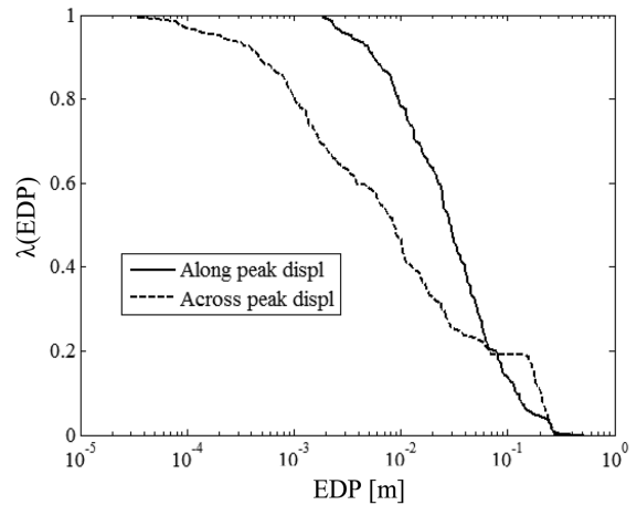
Fig. 7 Sensitivity analyses –set No. 4: mean annual frequencies \lambda(EDP) of exceeding any value of the considered EDP
