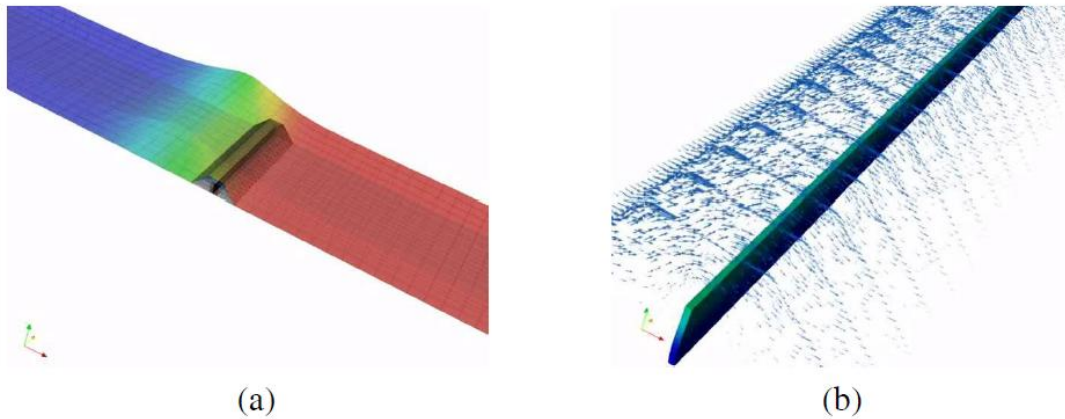
Fig. 7 (a) Wave, fluid at a fine scale and structure coupled. (b) Velocity field of the fluid at fine scale around the structure
