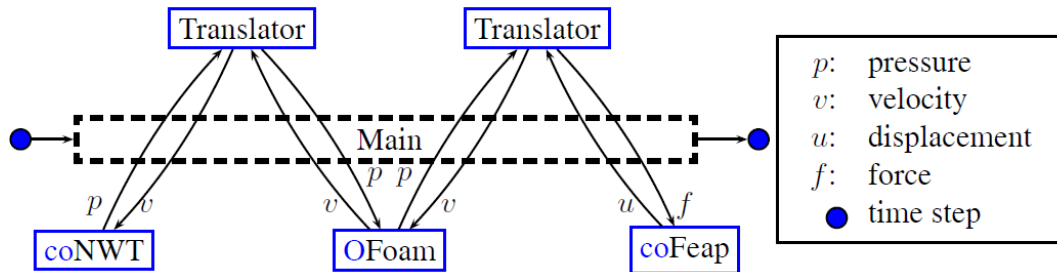
Fig. 2 Coupled three components for the BEM/VOF/FEM problem
