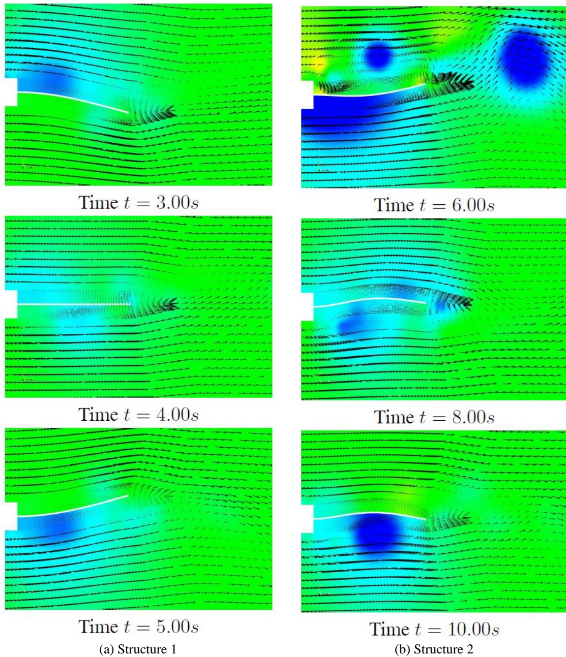
Fig. 5 Pressure and velocity fields in the fluid around the two structures considered
