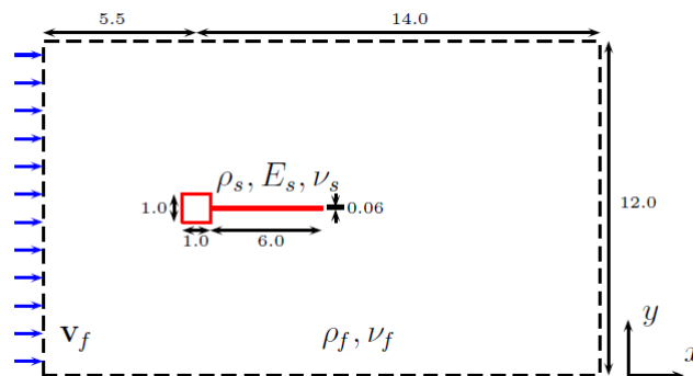
Fig. 3 The benchmark used for FSI problems
