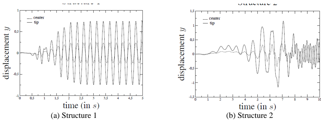
Fig. 4 Displacement following the y axe for the tip and center of the thin appendage. The scales are not the same on the two graphics
