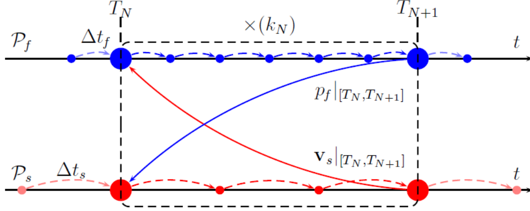
Fig. 1 Block Gauß-Siedel coupling algorithm for fluid ( P_f ) – structure ( P_s ) interaction problem; this iterative scheme is applied ( k_N ) times until the convergence is reached in a time window [T_N, T_{N+1}]
