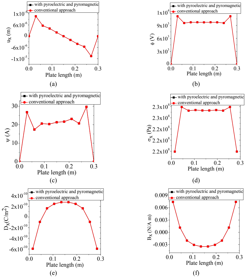
Fig. 4 Variation of (a) longitudinal x-direction displacement, (b) electric potential, (c) magnetic potential, and longitudinal x-direction (d) thermal stress, (e) electric displacement and (f) magnetic flux density
