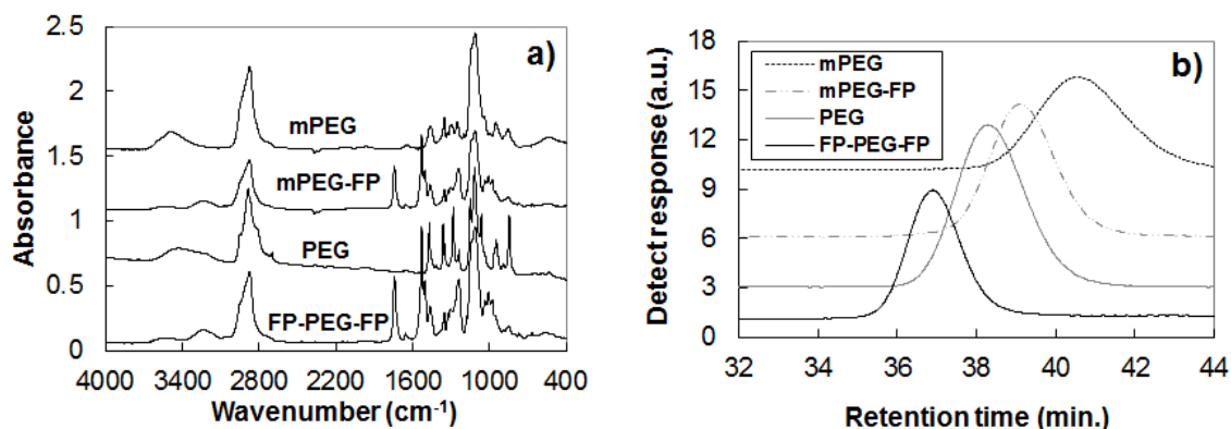
Fig. 2 FTIR (a) and gel permeation chromatograms (b) of mPEG (550 Daltons), mPEG-FP, PEG (1000 Daltons), and FP-PEG-FP
