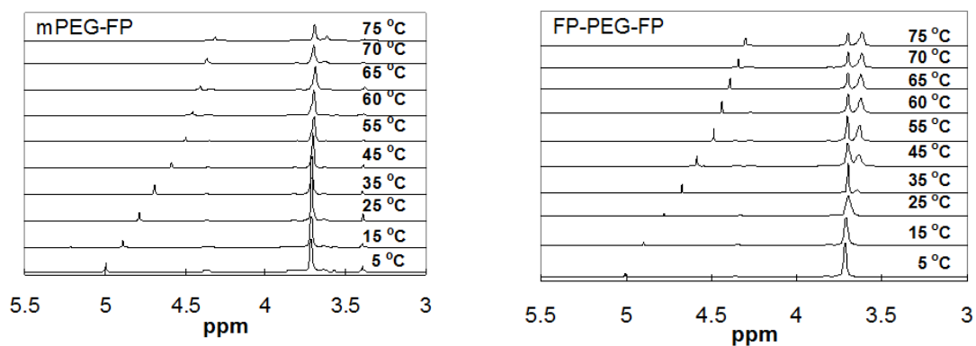
Fig. 4 1 H-NMR spectra (in D 2 O) of mPEG-FP and FP-PEG-PF as a function of temperature at 10.0 wt.%
