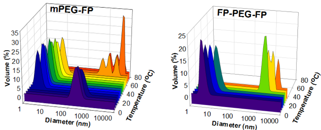
Fig. 5 Apparent size of mPEG, mPEG-FP, FP-PEG-PF at 10.0 wt.% determined by dynamic light scattering
