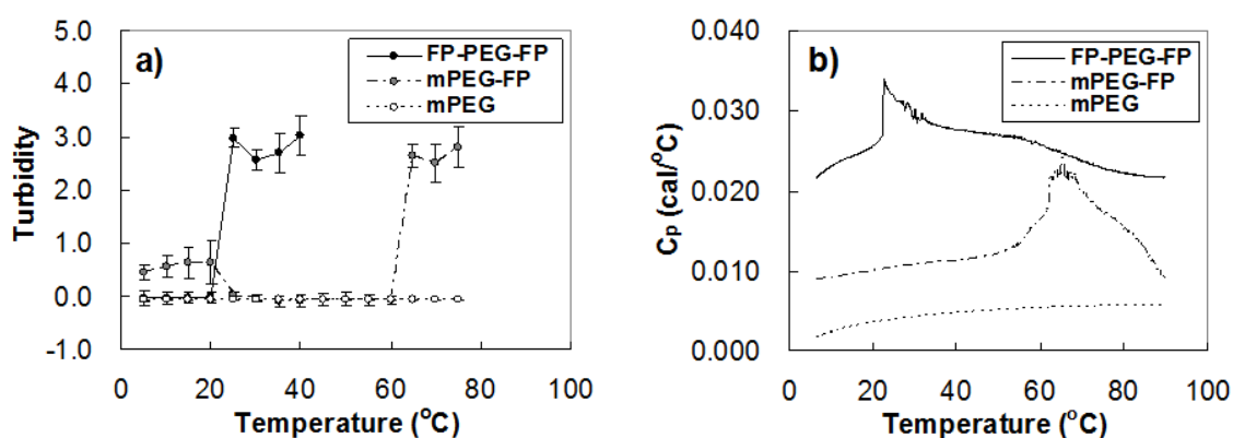
Fig. 3(a) Turbidity of mPEG, mPEG-FP, FP-PEG-PF as a function of temperature at 10.0 wt.%. The turbidity was defined as -\text{Log}(\text{transmittance}) at 550 nm (b) Microcalorimetric measurement of mPEG, mPEG-FP, FP-PEG-PF at 10.0 wt.%
