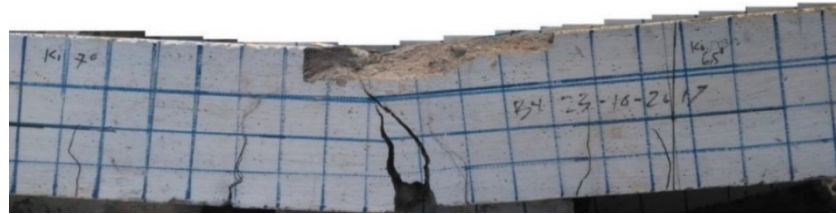
(a) B-PP-0.30
