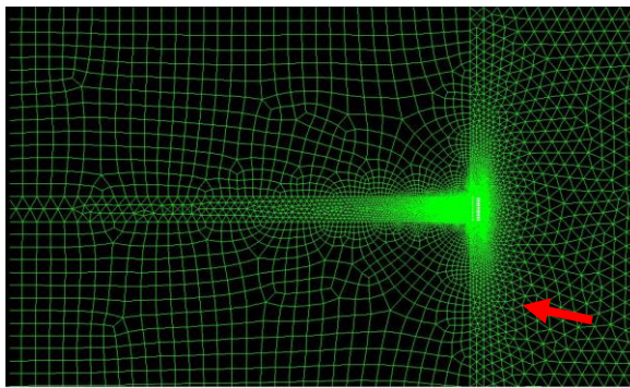
(a) Whole computational domain
