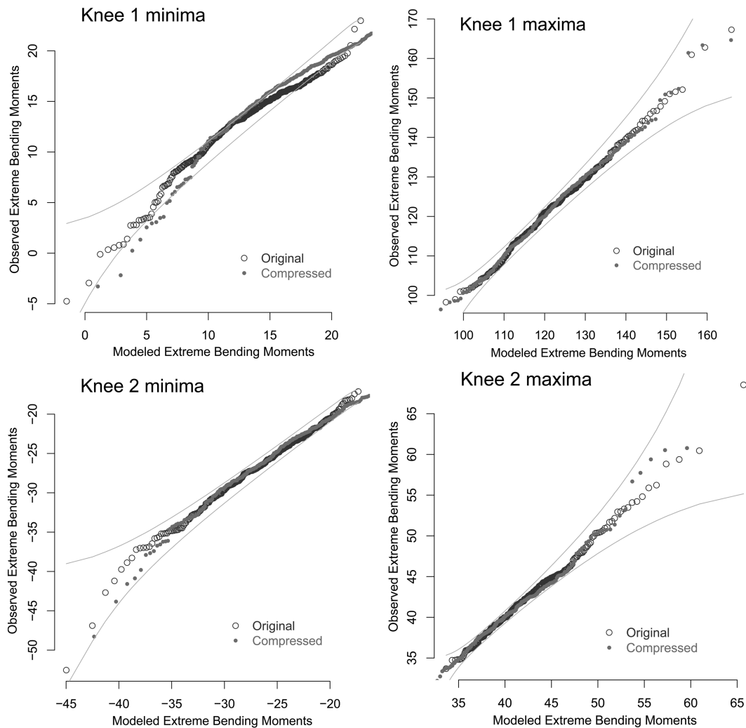
Fig. 6 Extreme bending moments before versus after compression. The ordinates of each plot are the observed extreme bending moments (in kNm) per unit of pressure (in \text{kN/m}^2 ) and unit of distance between frames (in m), for 20-min (full-scale) intervals. The abscissae are the expected values of a sample of the same size, drawn from a generalized extreme value (GEV) distribution fitted to the (blue) open circles, which correspond to the measured pressures. Since the parameters of the best fitting GEV distribution are different before and after compression, the abscissae of the (blue) open circles typically are different from the abscissae of the (red) dots in the same panel. The (red) dots correspond to the pressures reconstructed after 90% compression. The light-gray envelopes should enclose 99.5% of the samples, of the same size as those under consideration, that are drawn from the best fitting GEV distribution.
