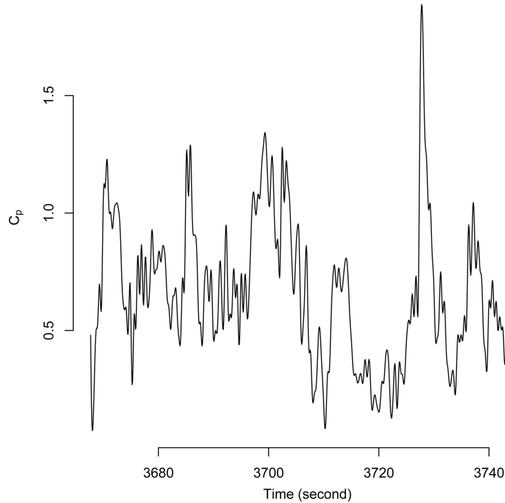
Fig. 3 C_p Fluctuations. Trace of 1,024 consecutive C_p values measured at tap 3, close to the end of run 48, shows a typical pattern: the fluctuations have no obvious periodicity, and are dominated by occasional sharp spikes (up or down) of very short duration, against a background that may drift over time.
