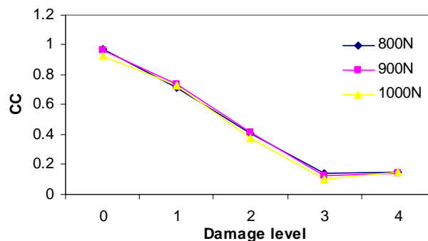
Fig. 10 CC index evaluated from conductance signatures (40 ~ 80 kHz) acquired from PZT patch surface-bonded on specimen C2 at different damage levels
