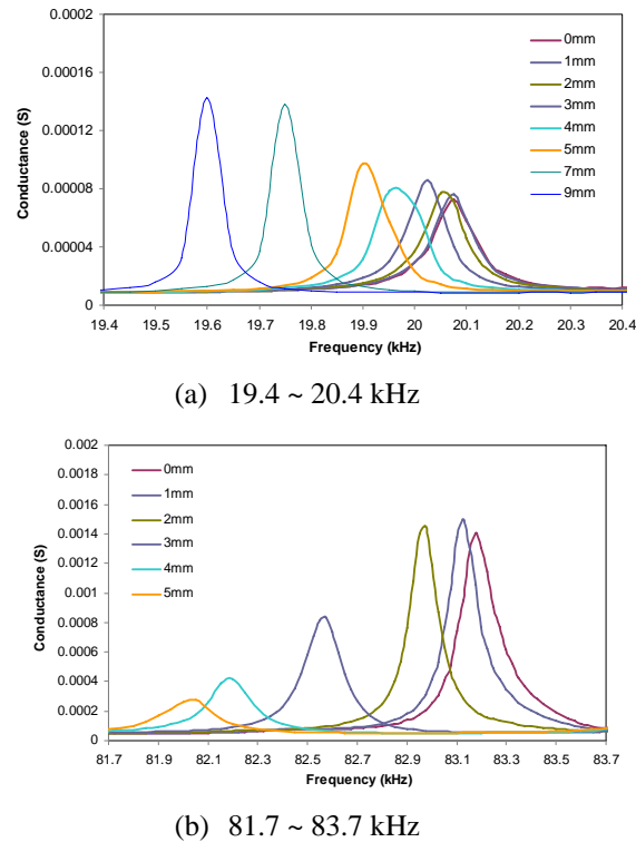
Fig. 6 Plot of conductance signatures versus frequency acquired from PZT patch surface-bonded on specimen T1 subjected to 3 kN tensile force at various crack length
