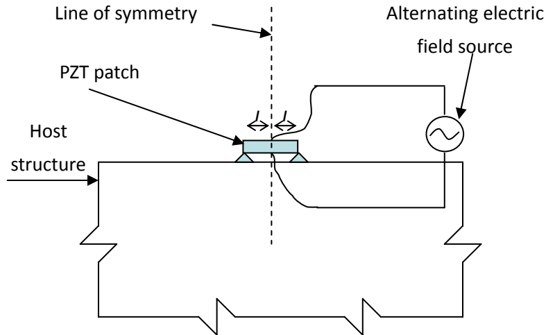
Fig. 1 Idealized interactions between a PZT patch and the host structure
