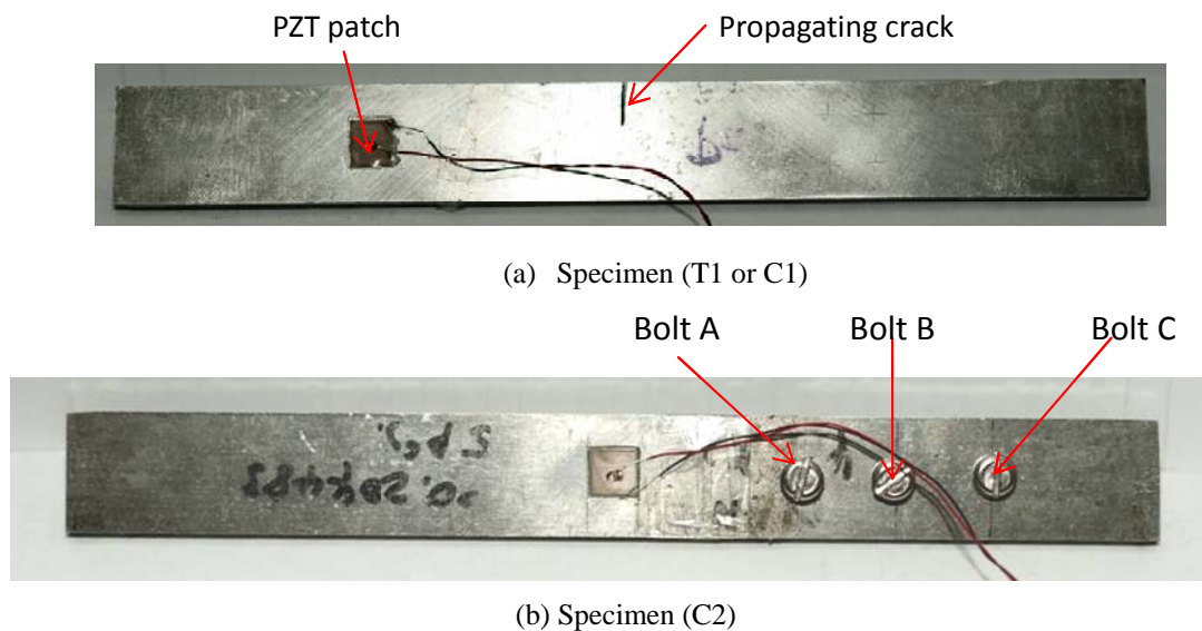
Fig. 2 Aluminum beam specimens (231 mm x 26 mm x 4 mm) of different configurations
