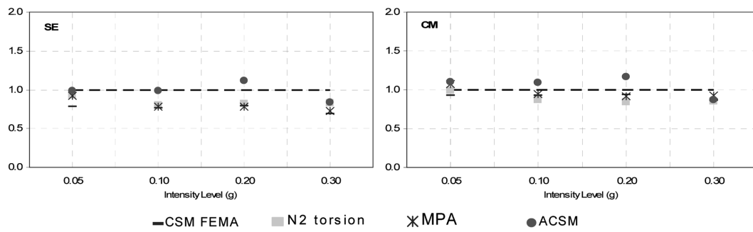
Fig. 13 Normalized roof displacements in the Y direction
