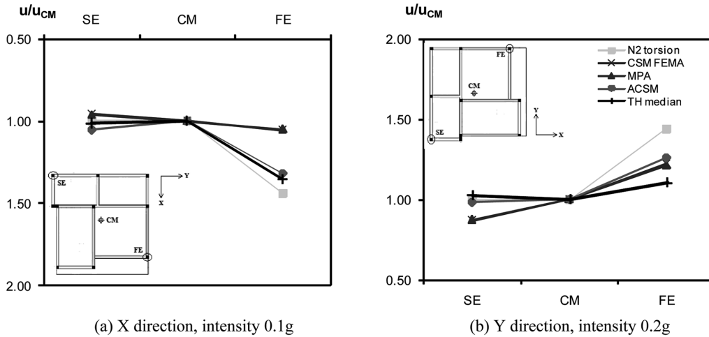
Fig. 15 Roof displacements normalized by CM displacement
