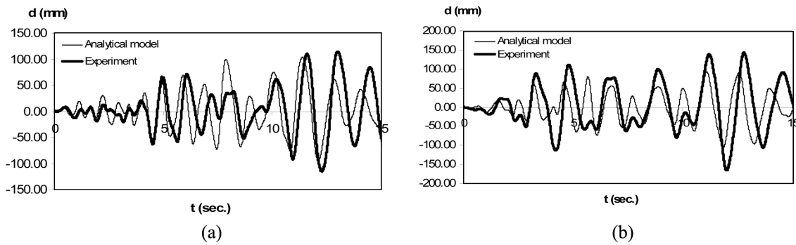
Fig. 3 (a) Top displacement in node C7, x-direction, (b) Top displacement in node N1, y-direction
