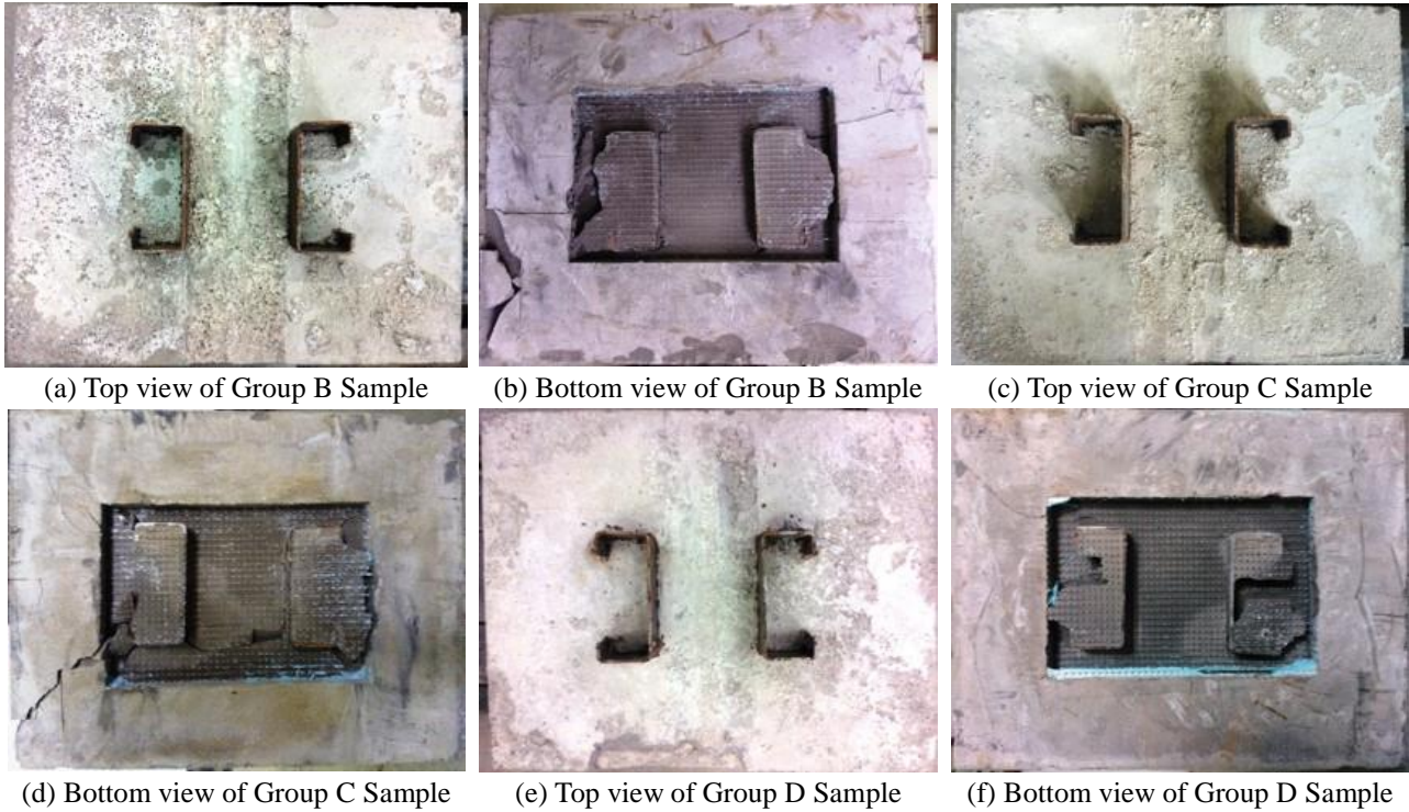
Fig. 8 Failure Modes of Group Specimens ((a), (c), and (e) are top surface and (b), (d), and (f) are bottom view of Groups B, C, and D, respectively)
