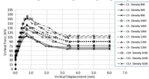
(c) Force displacement plot of group C specimens
