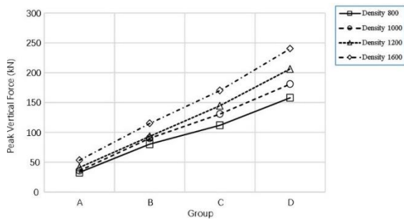
Fig. 6 Peak force for different groups of specimens
