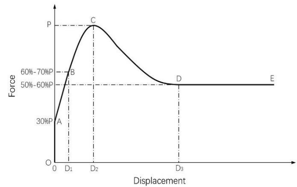
Fig. 4 Force and displacement behaviour curve
