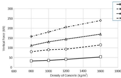
Fig. 5 Peak force versus foam concrete density
