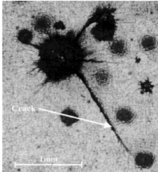
Fig. 1 Cracks in acrylic bone cement observed under transmitted light
