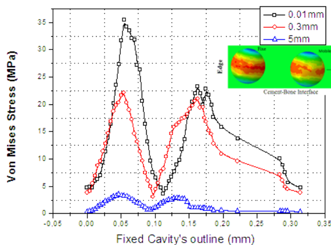
Fig. 9. Variation of the stress in cement around the mobile cavity according to the distance separating it to that fixed at the free edge both to the interface cement/bone
