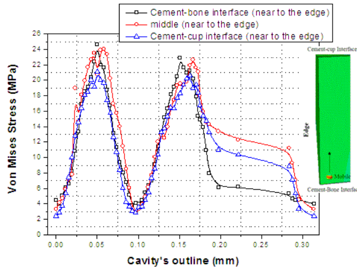
Fig. 7 Variation of the stress in the cement around the cavity according to its position along the thickness of the cement close to the edge
