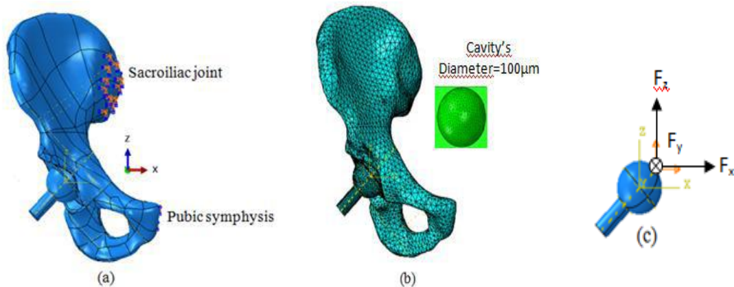
(a)Boundary condition and directions of forces applied to the center of femoral head (b)Meshed model of the pelvis and acetabular component (c) The three force components ( F_x, F_y, F_z )
