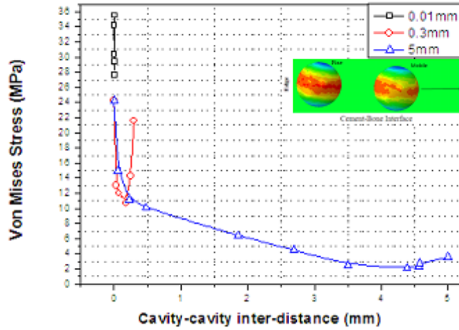
Fig. 10 Variation of the stress according to the fixed cavity- mobile cavity interdistance
