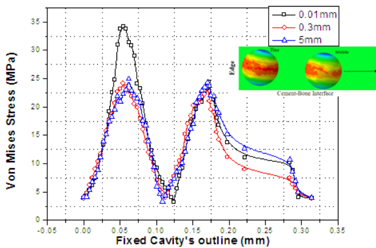
Fig. 8 Variation of the stress in the cement around the fixed cavity at the free edge according to the distance separating it to that mobile both to the interface cement/bone
