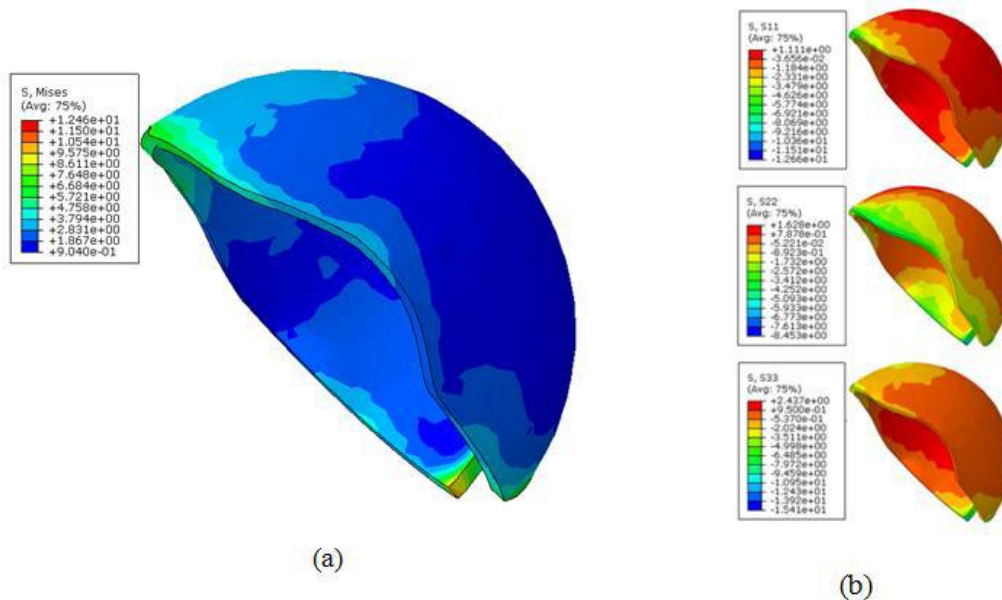
(a) Von Mises stress (b) Normal stresses Fig.4 Stress level and distribution in the cement
