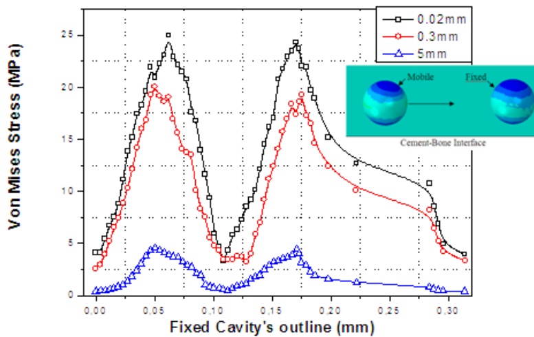
Fig. 11 Variation of the stress around the mobile cavity according to the distance separating it to that fixed both at the interface cement/bone
