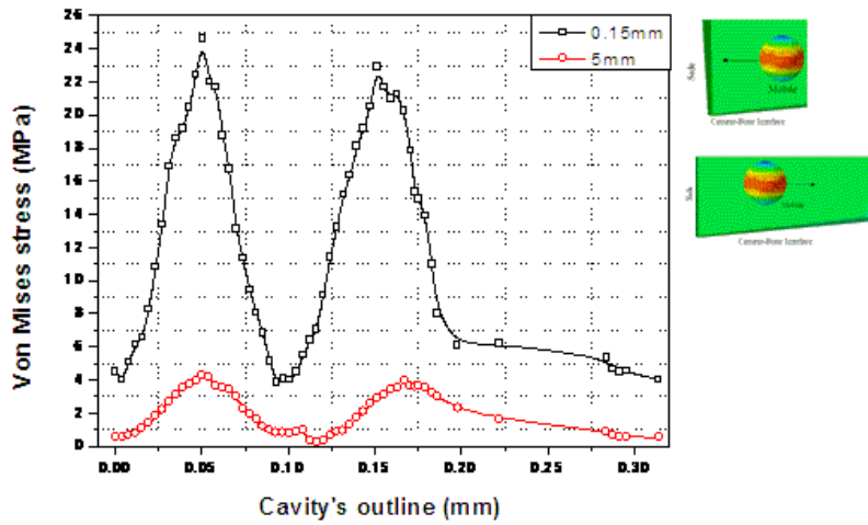
Fig. 6 Stress level and distribution in the cement around the cavity
