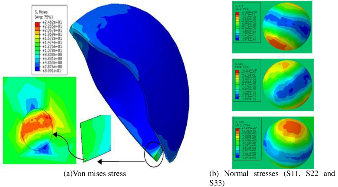
Fig. 5 Stress level and distribution in the cement around the cavity
