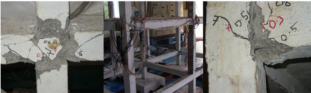
Fig. 21 Damage patterns observed at PGA = 0.7 g
